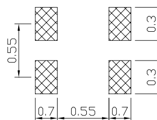
PCB PATTERN
