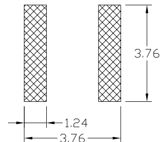
PCB PATTERN
