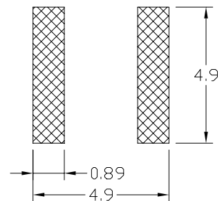
PCB PATTERN
