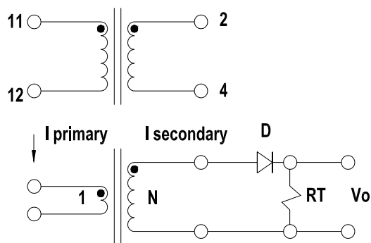
APPLICATION CIRCUIT
